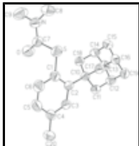
Fig. 1. Molecular structure of (I) with atom numbering scheme. Thermal ellipsoids are shown at the 50% probability level.
