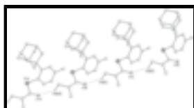
Fig. 2. View of the chains of (I) along the 001 axis.
